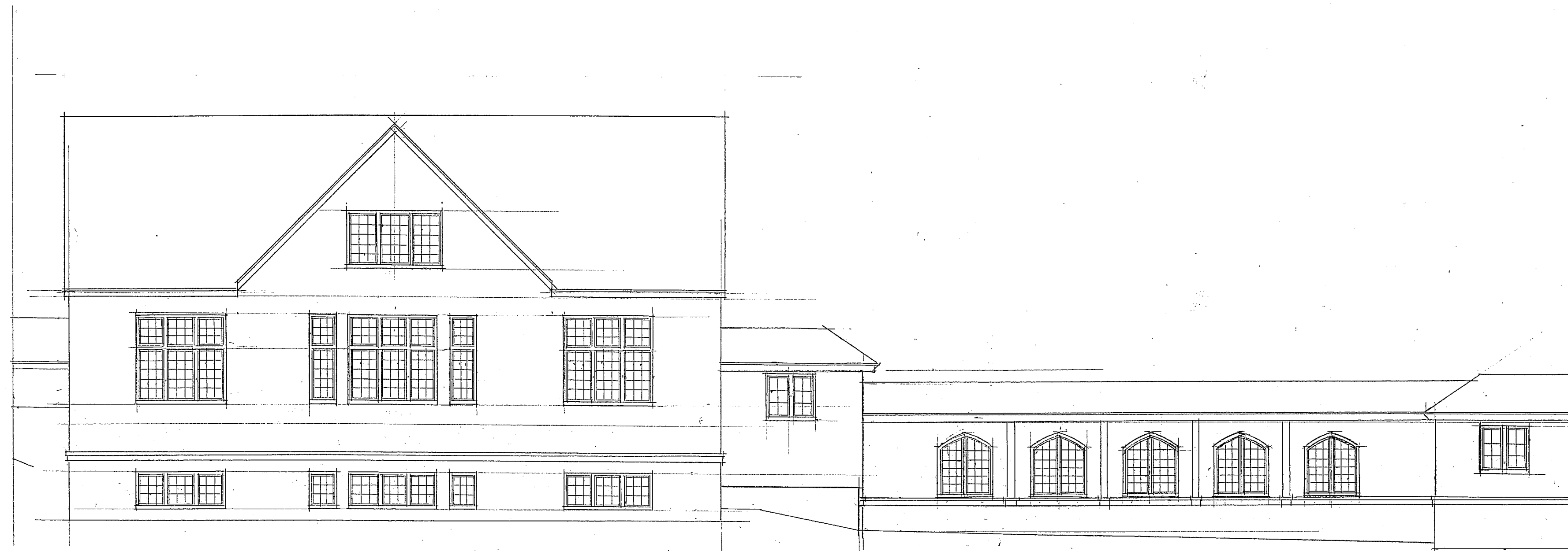
SOUTH ELEV. (BALTO BLDG, EAST ARCADE)
